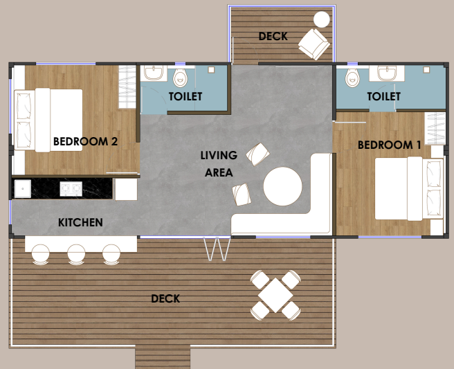
2 BHK TWO CONTAINER LAYOUT
