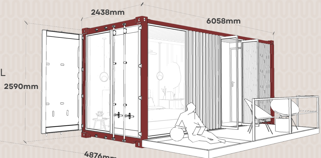
20' X 8' DOUBLE CONTAINERS MODEL
